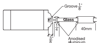
ALUMINUM GRILL SIDERAIL
