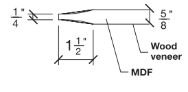
PANEL 5/8"
