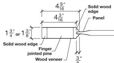
SIDERAIL
