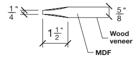
PANEL
