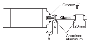
ALUMINUM GRILL SIDERAIL
