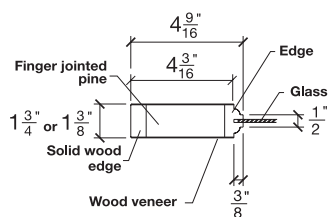
SIDERAIL
