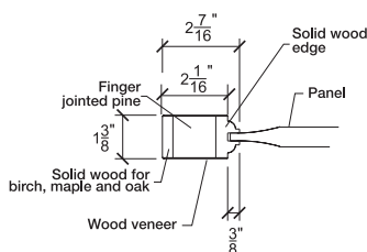
SIDERAIL 1 3/8"
