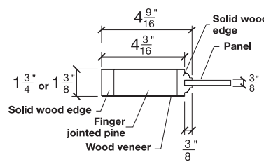
SIDERAIL
