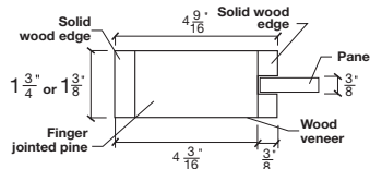
SHAKER SIDERAIL
