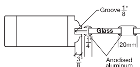
ALUMINUM GRILL SIDERAIL
