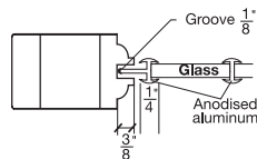
SIDERAIL 1 3/8"
