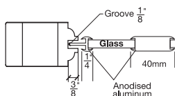
ALUMINUM GRILL SIDERAIL 1 3/8"
