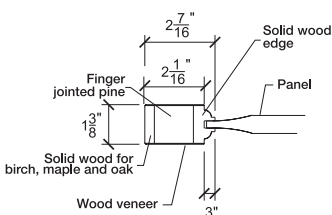
SIDERAIL 1 3/8"
