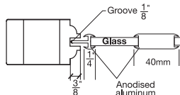
ALUMINUM GRILL SIDERAIL 1 3/8"
