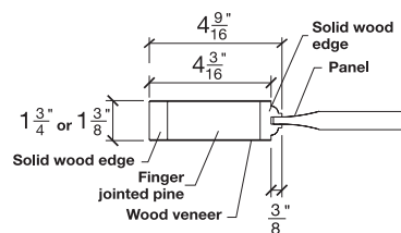
SIDERAIL
