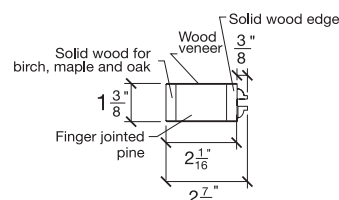
SIDERAIL 1 3/8"
