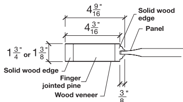
SIDERAIL
