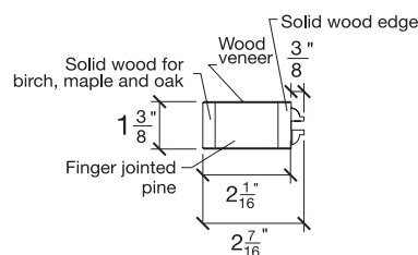
SIDERAIL 1 3 3/8"
