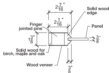
SIDERAIL 1 3/8"
