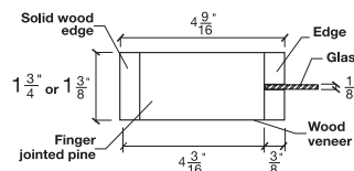
SHAKER SIDERAIL
