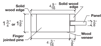
SHAKER SIDERAIL
