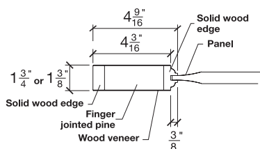
SIDERAIL
