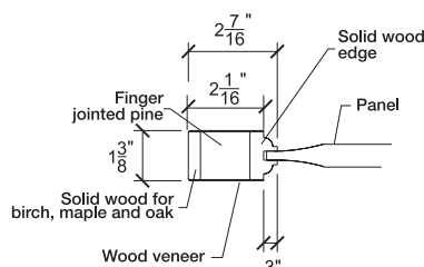
SIDERAIL 1 3/8"
